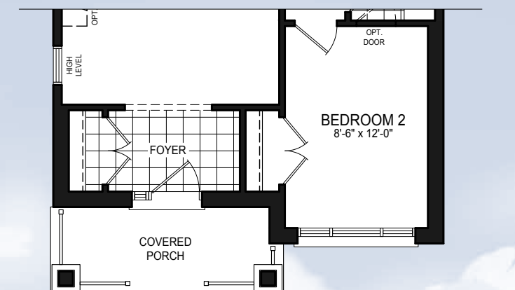
Optional 2 Bedroom Ground Floor Elevation B
