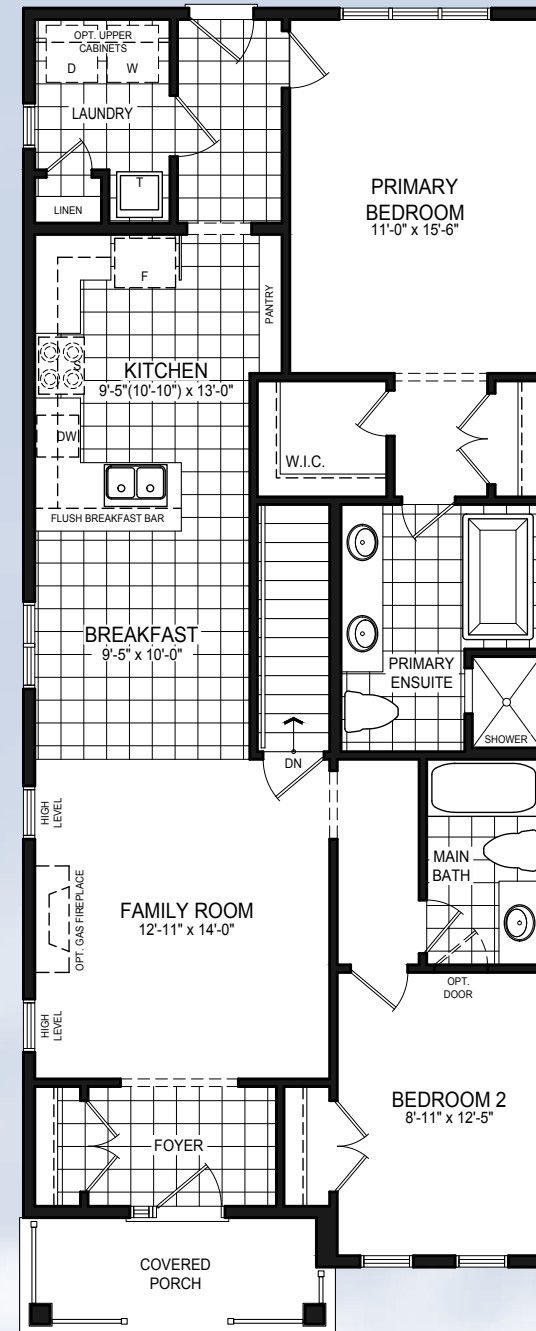
Optional 2 Bedroom Ground Floor Elevation A
