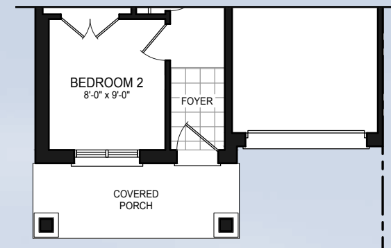
Ground Floor Elevation B1 & B2
