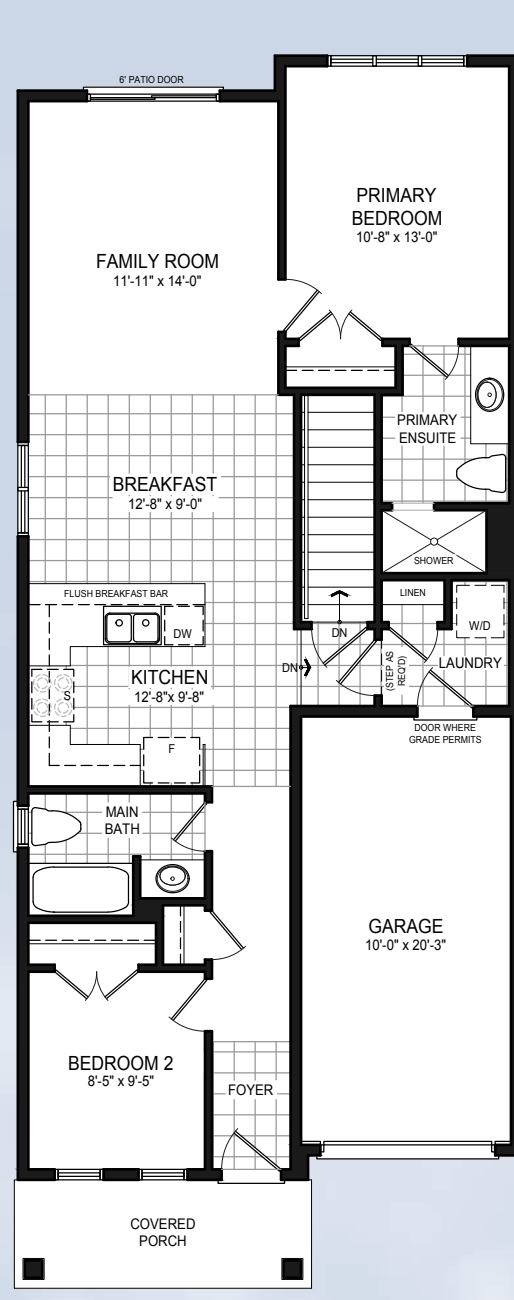
Ground Floor Elevation A1 & A2
